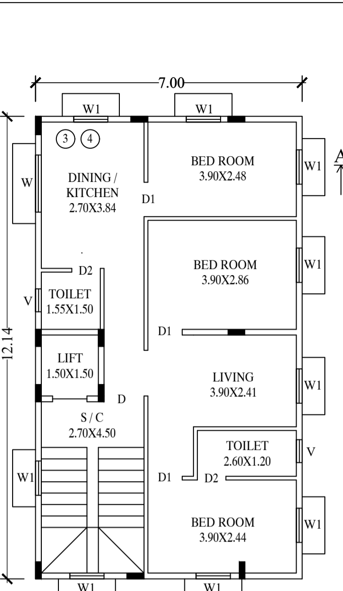
PROPOSED TYPICAL FIRST & SECOND FLOOR PLAN
